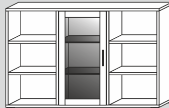
00089L/40/F/G* 134x86x40cm (BxHxT) 00089L/32/F/G* 134x86x32cm (BxHxT)
