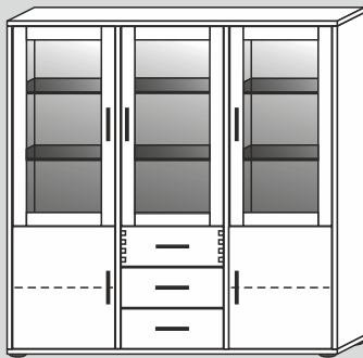
00022L/40/F/G* 134x134x40cm (BxHxT) 00022L/32/F/G* 134x134x32cm (BxHxT)
