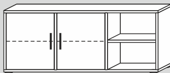
00027L/40/F/G* 134x54x40cm (BxHxT) 00027L/32/F/G* 134x54x32cm (BxHxT)
