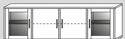
00045/40/F/G* 178x54x40cm (BxHxT) 00045/32/F/G* 178x54x32cm (BxHxT)
