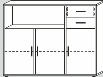
00024L/40/F/G* 134x102x40cm (BxHxT) 00024L/32/F/G* 134x102x32cm (BxHxT)
