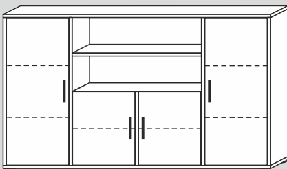
00027/40/F/G* 178x102x40cm (BxHxT) 00027/32/F/G* 178x102x32cm (BxHxT)
