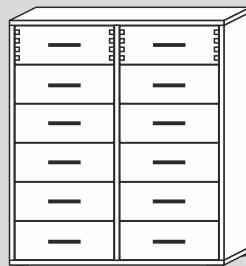
00052/40/F/G* 90x102x40cm (BxHxT) 00052/32/F/G* 90x102x32cm (BxHxT)
